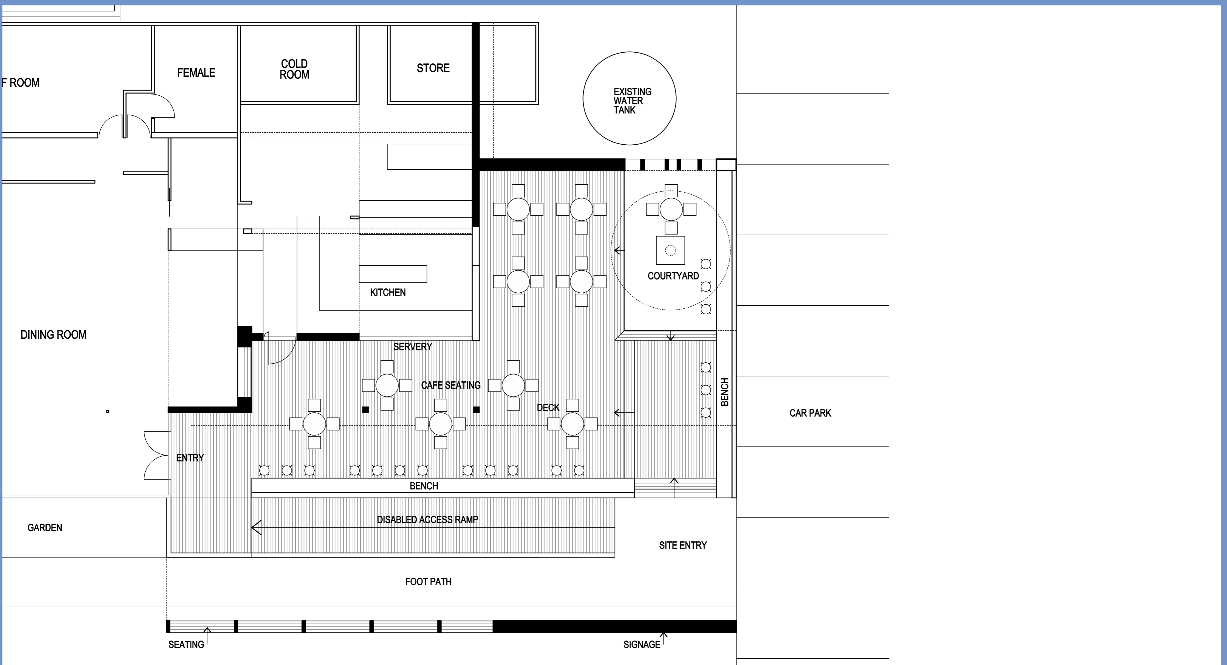
Brisbane Racing Sports & Social Club New Terrace Floor Plan
